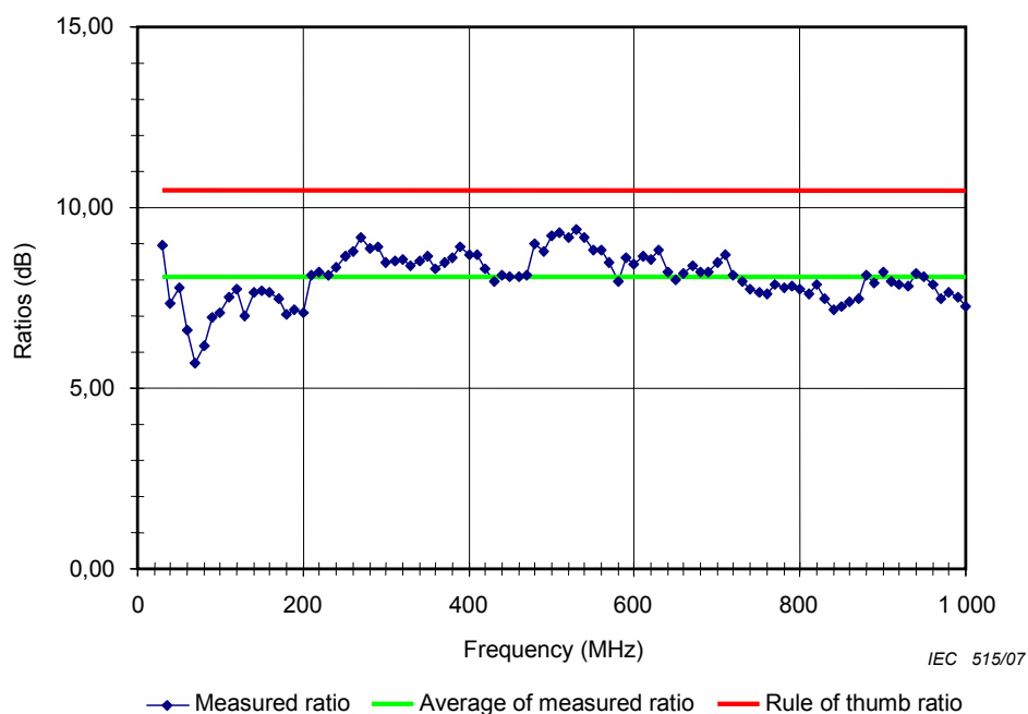
Figure F.5 – Measured correlation curve of 3 m and 10 m SAC/OATS-emission measurement of a battery-fed table-top type of EUT, compared with the free-space rule-of-thumb ratio [f7], [f8]
