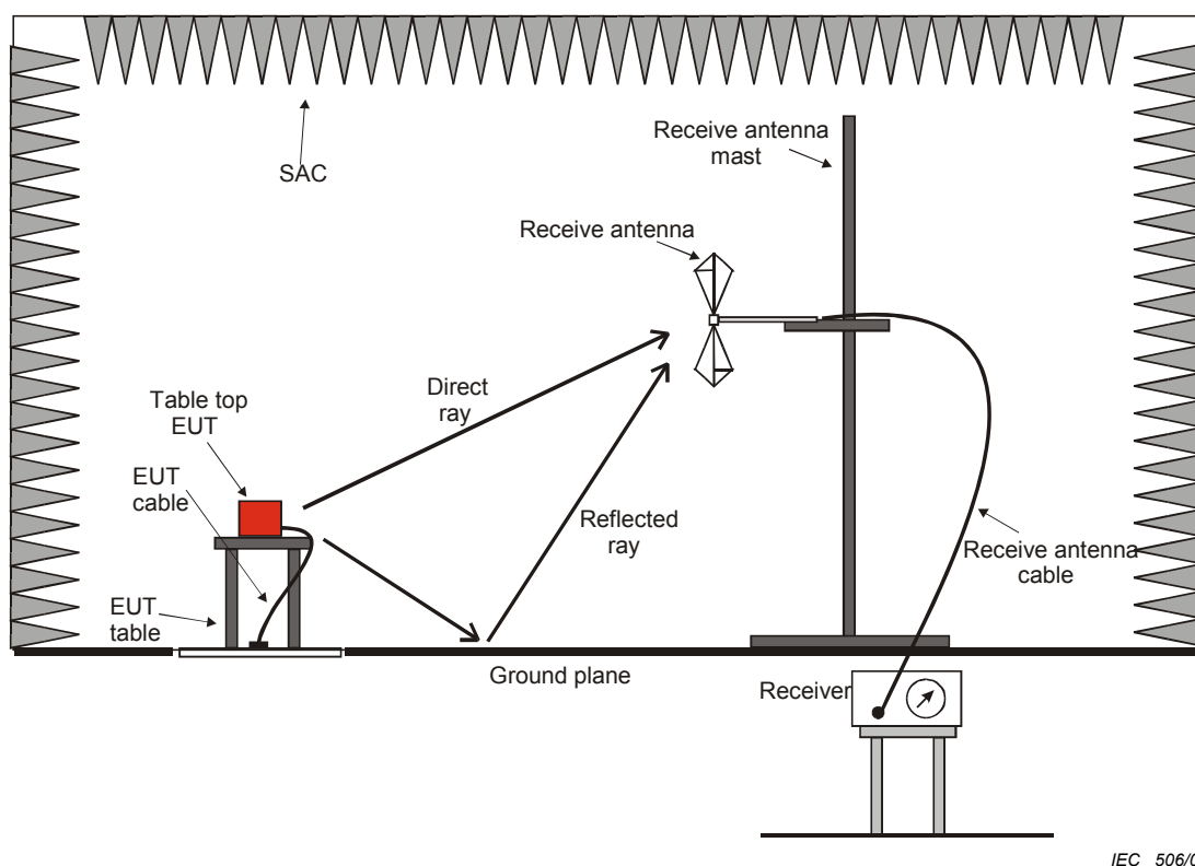
Figure 8-1 – Schematic of a radiated emission measurement set-up in a SAC
