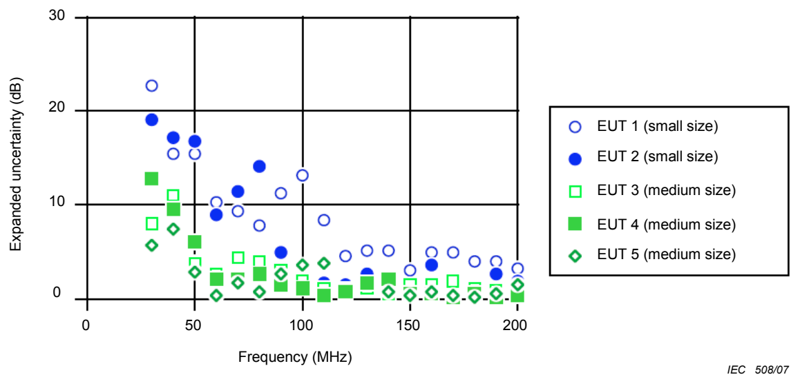
Figure F.1 – Expanded uncertainties of emission measurement results for five different emulated EUTs each with five different cable termination conditions [f2]
